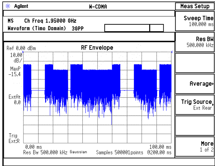
Displayed Compressed Signal and Signal Parameters
