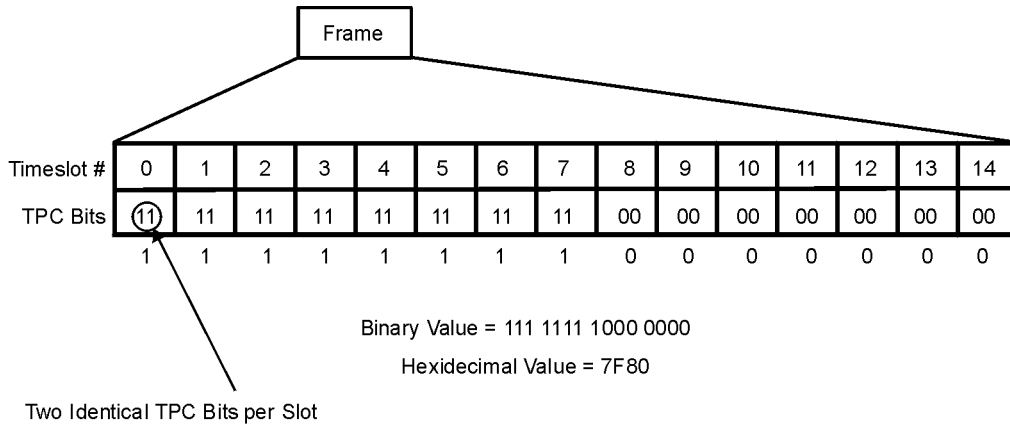
Figure 15-11 TPC Bits per Timeslot
