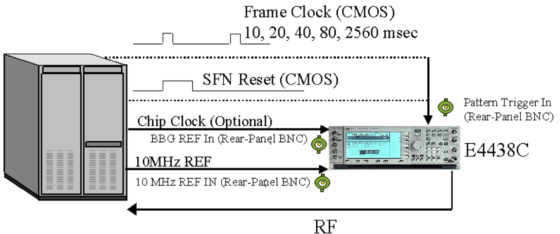
Figure 16-73 Cable Connections
