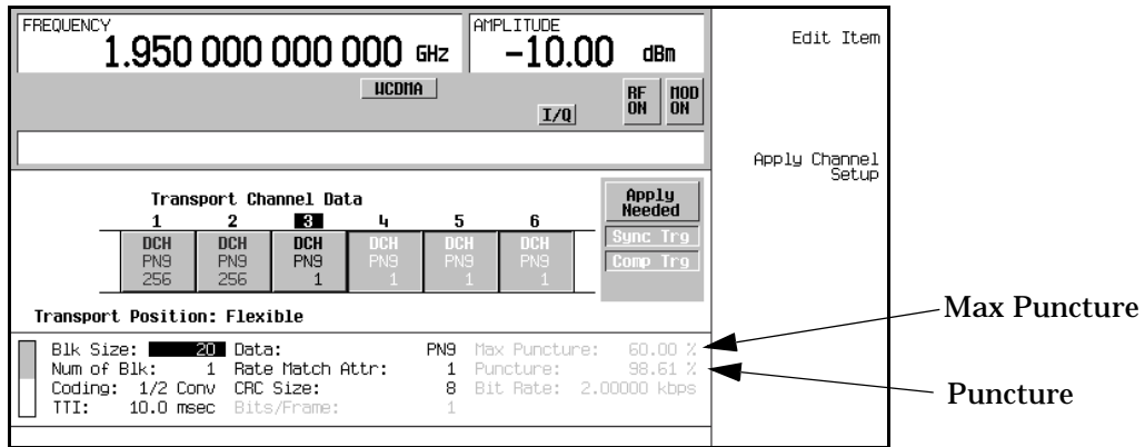
Figure 16-41 Excessive Puncturing
