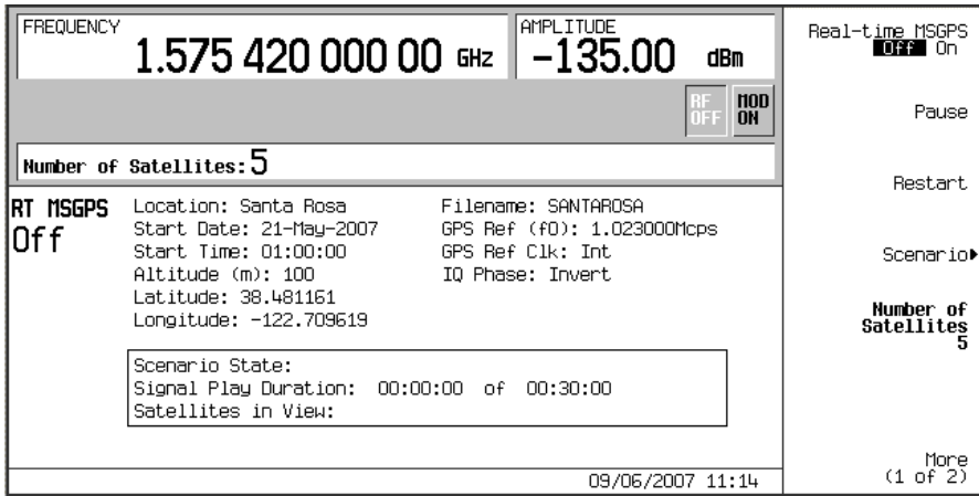
Figure 11-2 Real Time MSGPS Scenario
