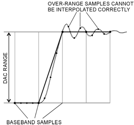
Figure 4-25 Waveform Overshoot
