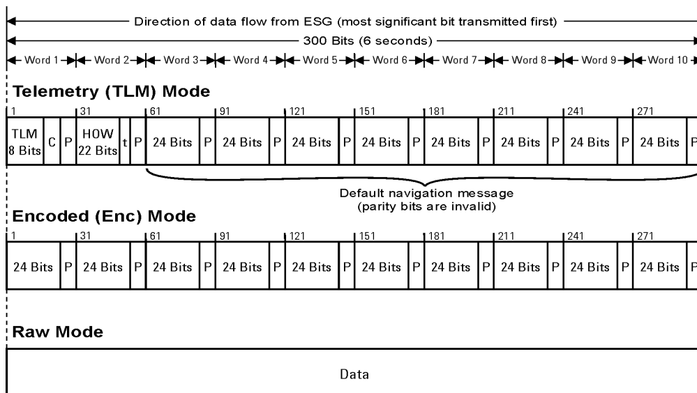
Figure 11-4 Subframe Structures
