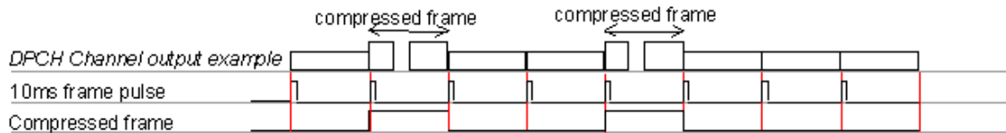
Figure 16-76 DPCH Signal Alignment
