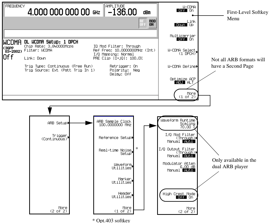
Figure 4-14 ARB I/Q Filters and Attenuator Softkey Location
