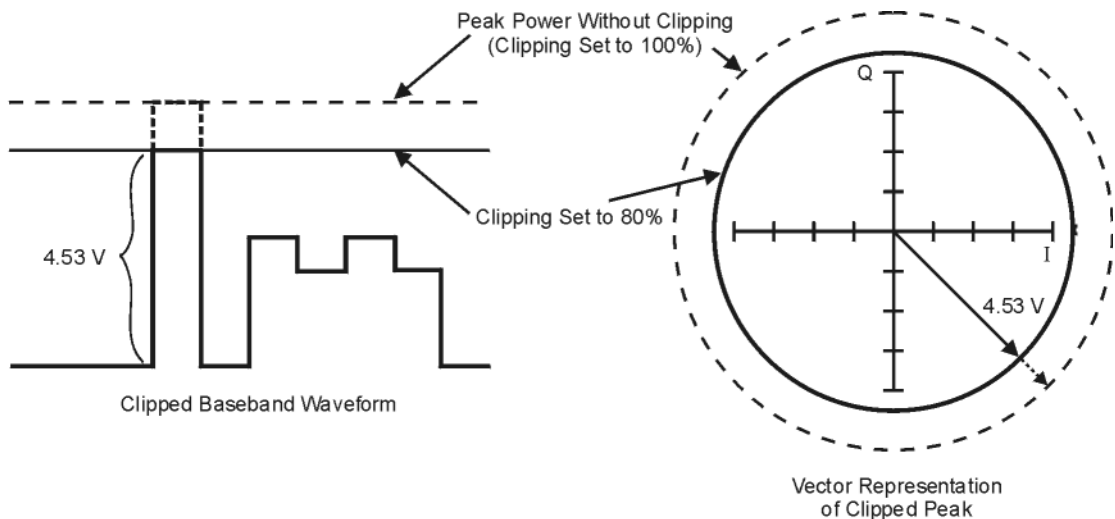
Figure 4-21 Circular Clipping
