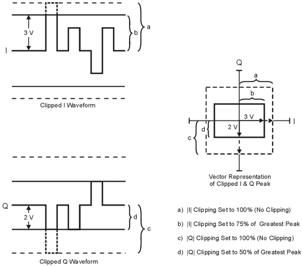
Figure 4-22 Rectangular Clipping
