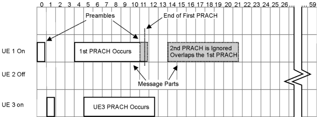
Figure 16-21 Transmitting PRACHs
