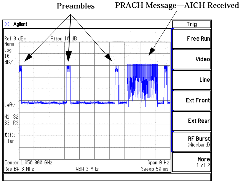
Displayed ESG Signal
