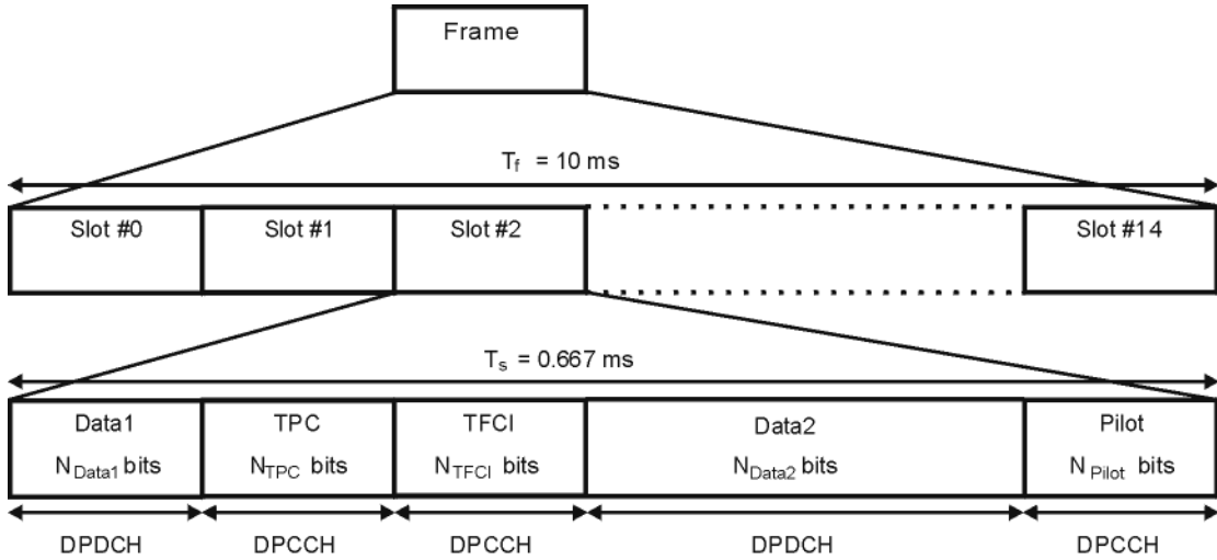
Figure 15-19 DPCCCH/DPDCH Frame Structure
