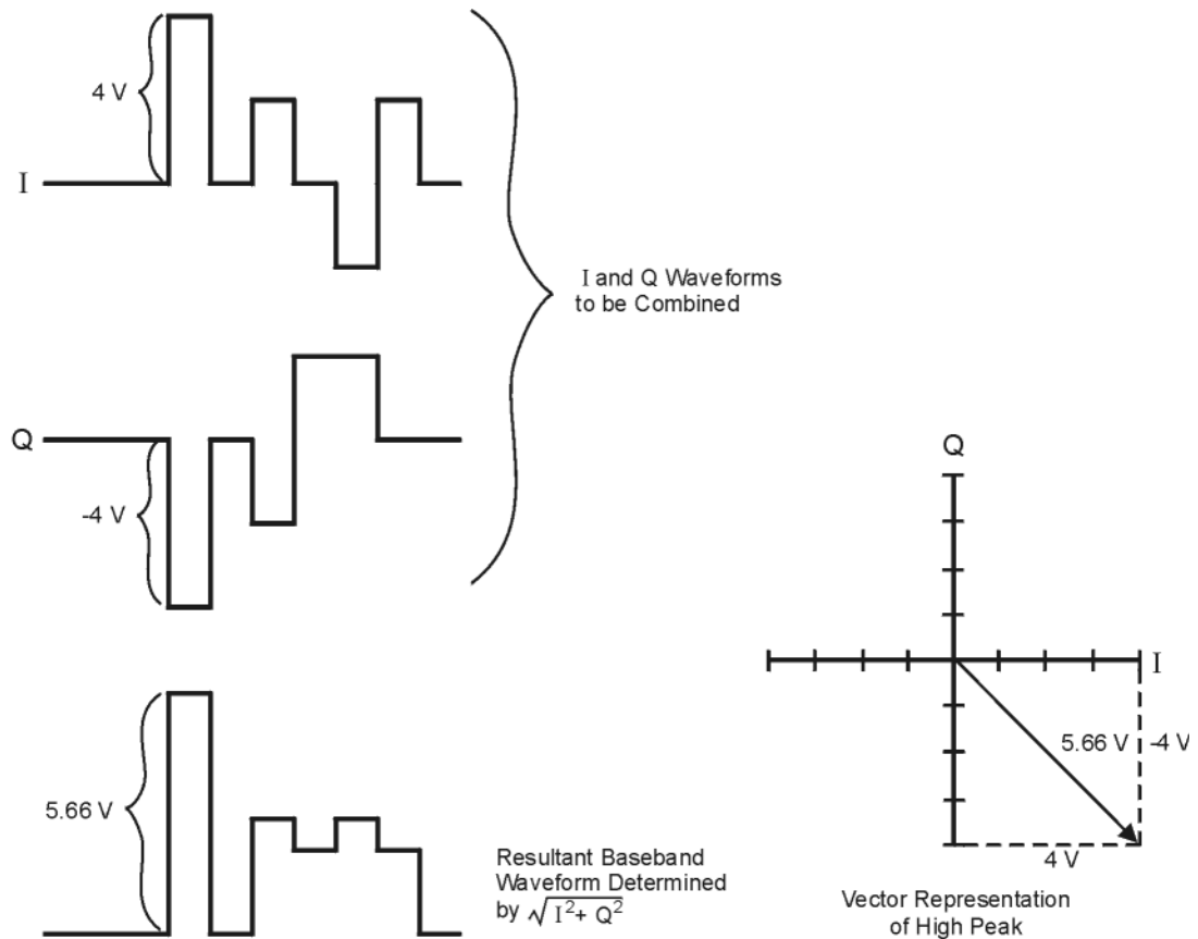
Figure 4-18 Combining the I and Q Waveforms
