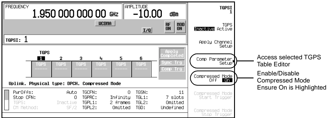
Figure 16-58 TGPSI Display
