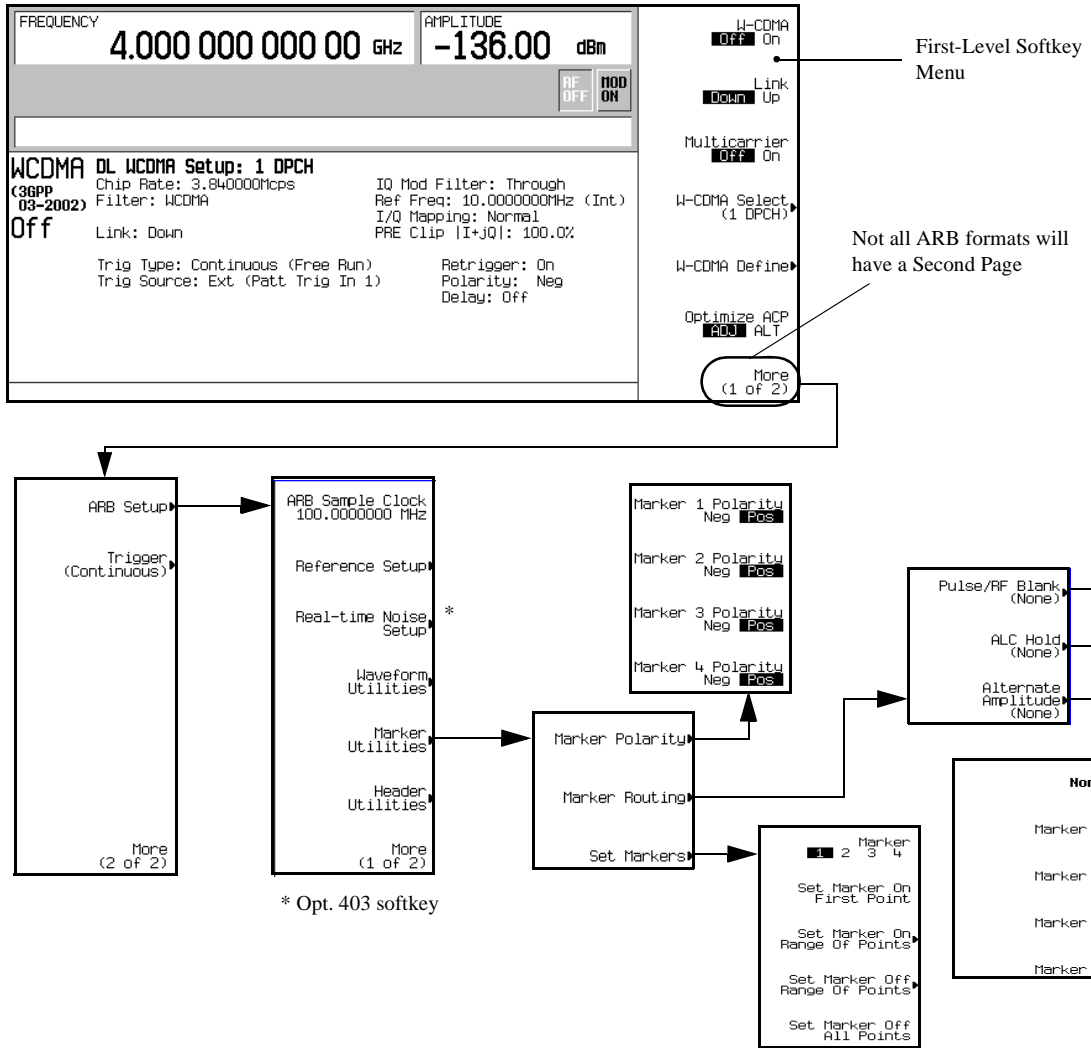
Figure 4-15 ARB Marker Location and Softkey Menus
