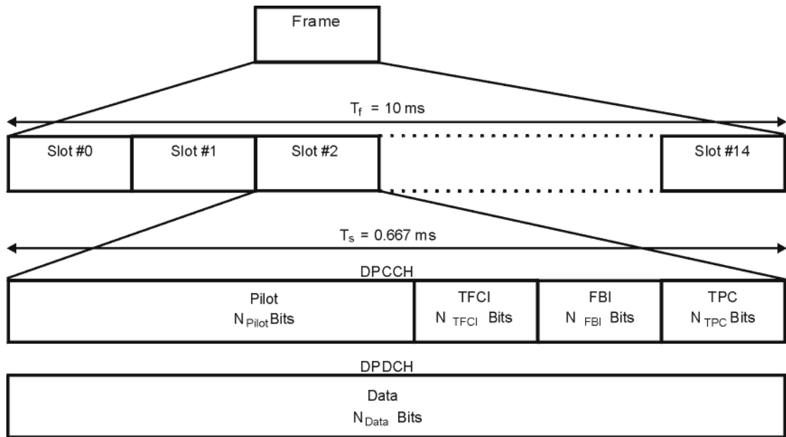
Figure 16-90 DPCCH/DPDCH Frame Structure
